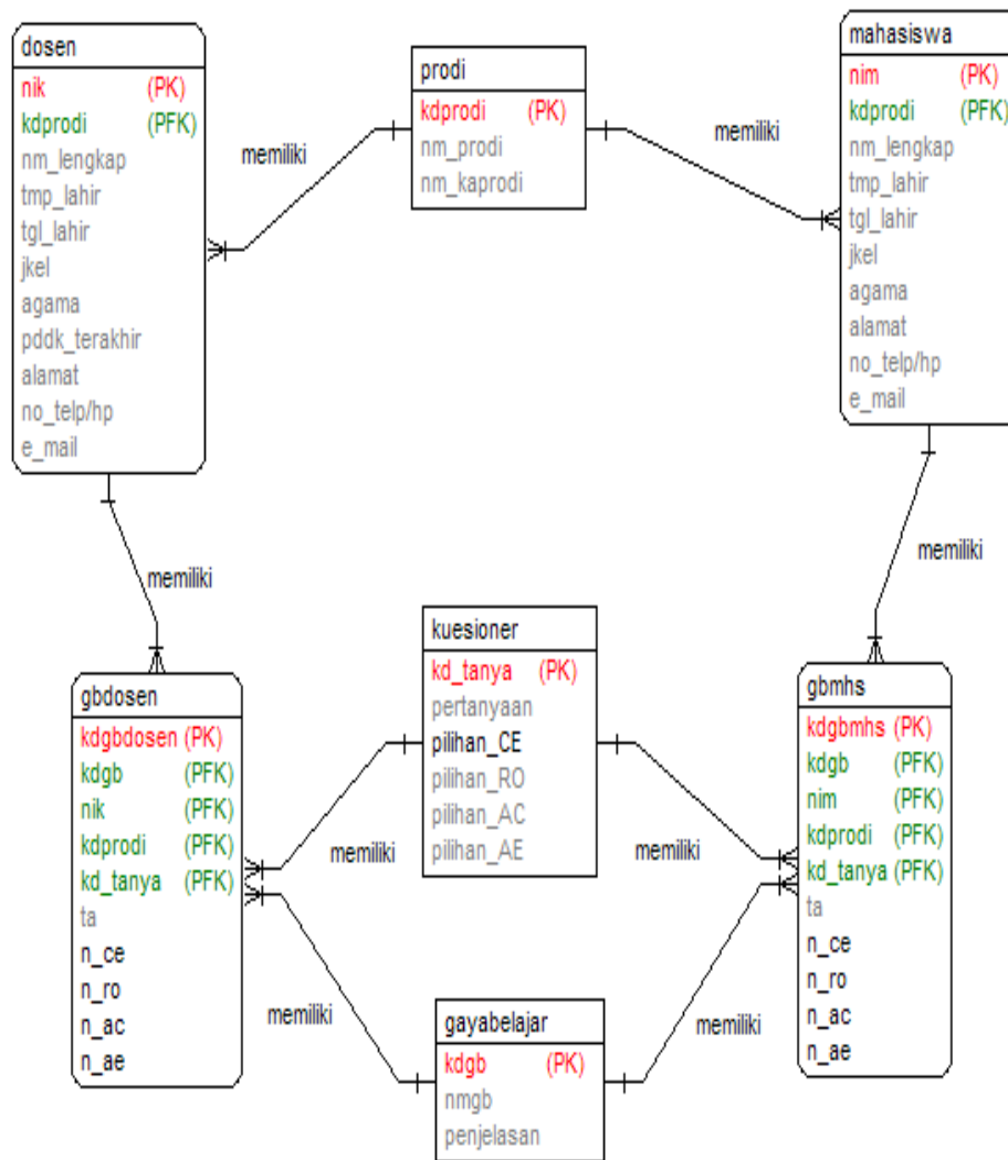
Gambar 2 Entity Relationship Diagram
