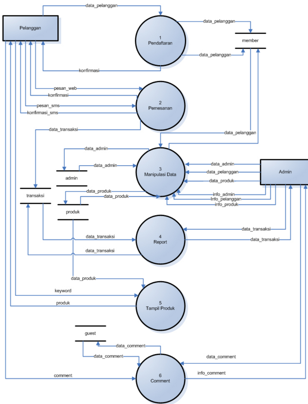
Gambar 4 DFD Level 0
